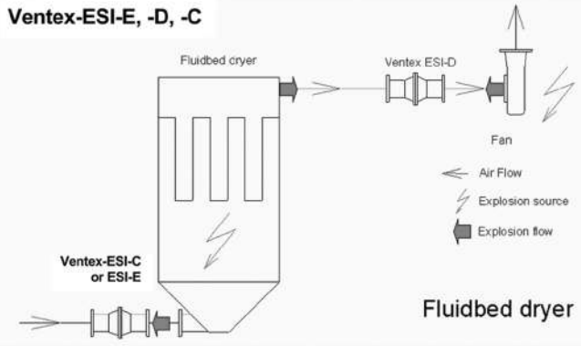
Figure 33 Setup of fluid bed with different Ventex valves. (Courtesy of Rico-Sicherheitstechnik AG, Switzerland.)
