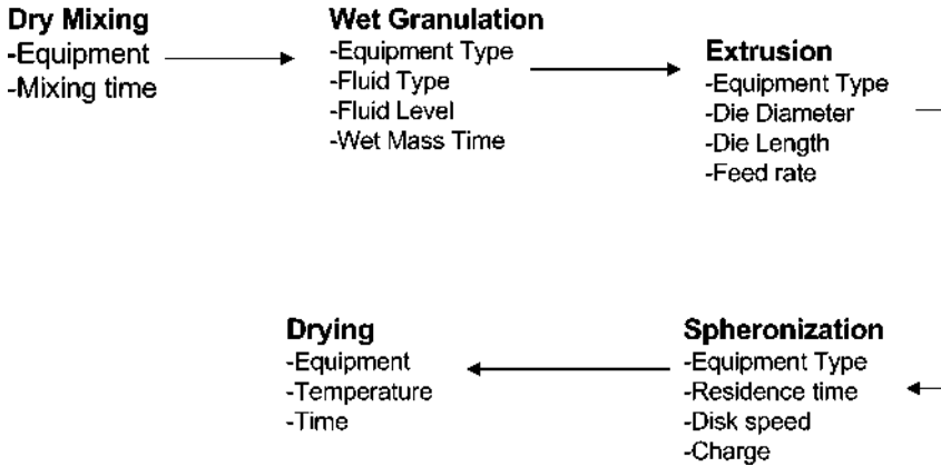
Figure 2 Process flow chart of the extrusion/sphronization process showing the process variables for each individual step. (From Ref. 24.)
