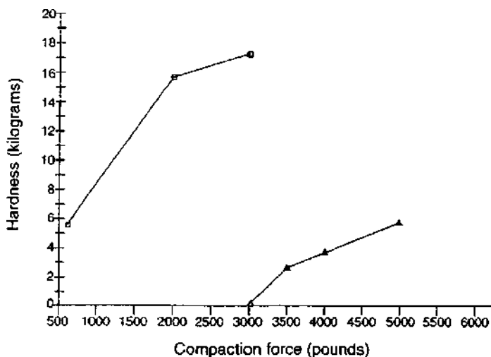
Figure 21 The effect of varying compression force on the hardness of compacted 16/30-mesh spheres of 10% theophylline-Avicel PH101: \Delta , spheres prepared by water; \square , spheres prepared by 95% ethanol granulation. (From Ref. 18.)
