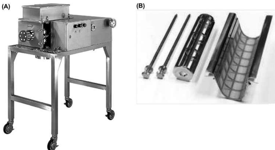
Figure 1 Oscillating granulator: (A) Frewitt MF line and (B) rotor, screen, and tensoning spindles.
