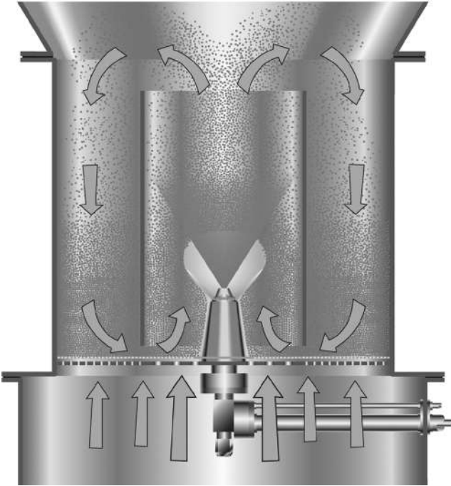
Figure 40 (A) Wurster Coater schematic. (B) Wurster Coater. (Courtesy of the Vector Corporation.)
