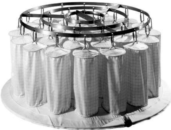
Figure 12 Conventional bag filters with hanging arrangements. (Courtesy of the Vector Corporation.)
