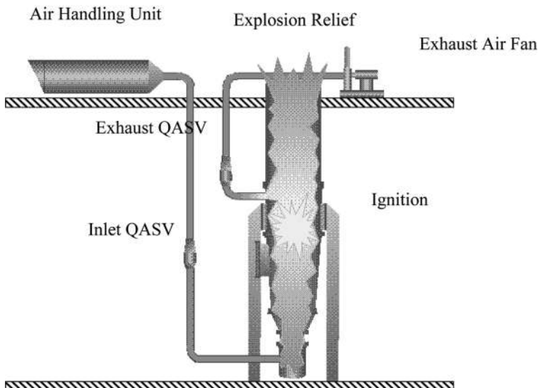
Figure 30 Vented design (2 bar unit). (Courtesy of the Glatt Group.)
