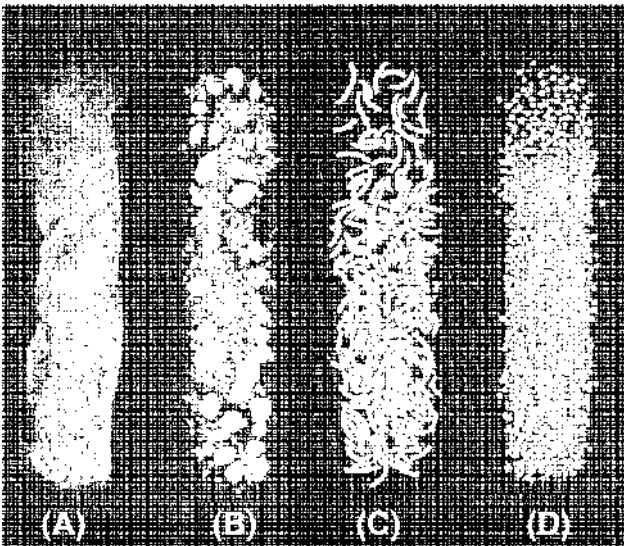
Figure 3 Product produced by the first four extrusion/sphronization process steps. (A) Powder from dry mixing; (B) granules from granulation; (C) extrudate from extrusion; and (D) spheres from sphronization.
