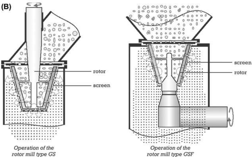
Figure 3 Conical-screening mill: (A) Glatt model GSF 180 and (B) principle of operation.
