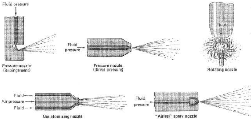
Figure 7 Types of nozzle. (From Ref. 29.)
