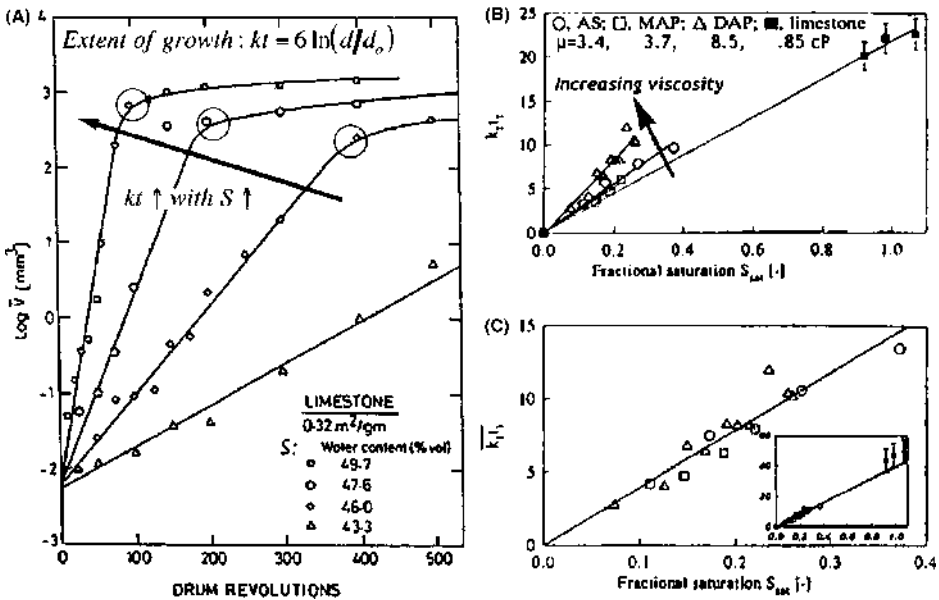
Figure 40 (A) Exponential growth in drum granulation reaching a growth limit d_{\max} , or maximum extent of growth (kt)_{\max} , which are functions of moisture saturation (15–19). (B) Maximum extent of noninertial growth (kt)_{\max} as a linear function of saturation of the powder feed and binder viscosity. (C) Maximum extent normalized for differences in binder viscosity, drum speed, granule density by Stokes number. (From Ref. 46.)
