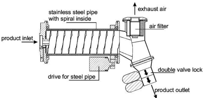
Figure 14 Sectional sketch of a contact dryer.
