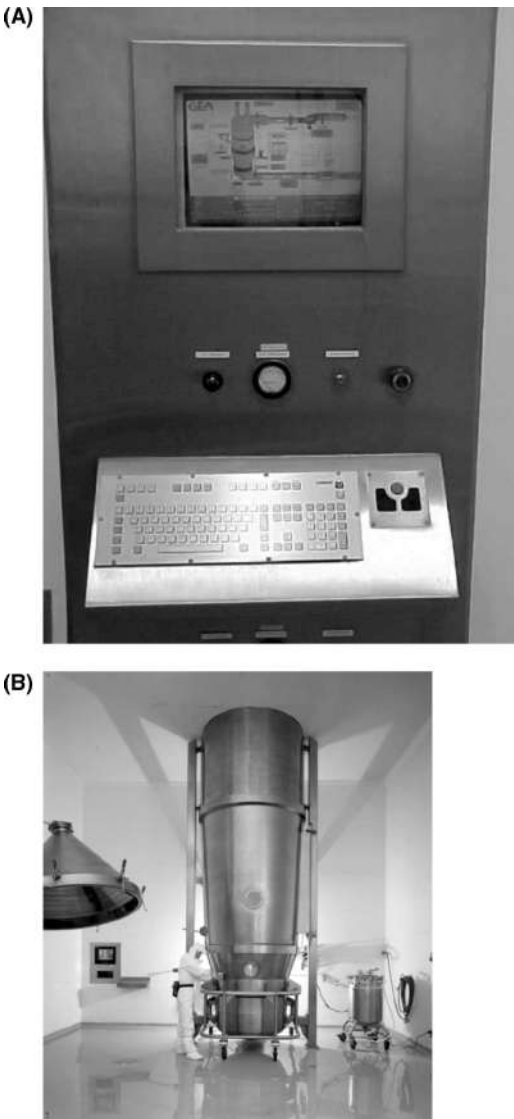
Figure 26 (A) PLC based system. (Courtesy of Niro Pharma Systems.) (B) Production unit with a PLC control panel. (Courtesy of the L.B. Bohle Group.)
