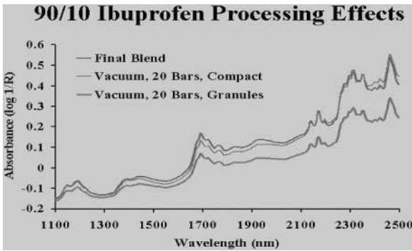
Figure 22 NIR absorbance 90/10 Ibuprofen/Starch processing effects. (From Ref. 39.)
