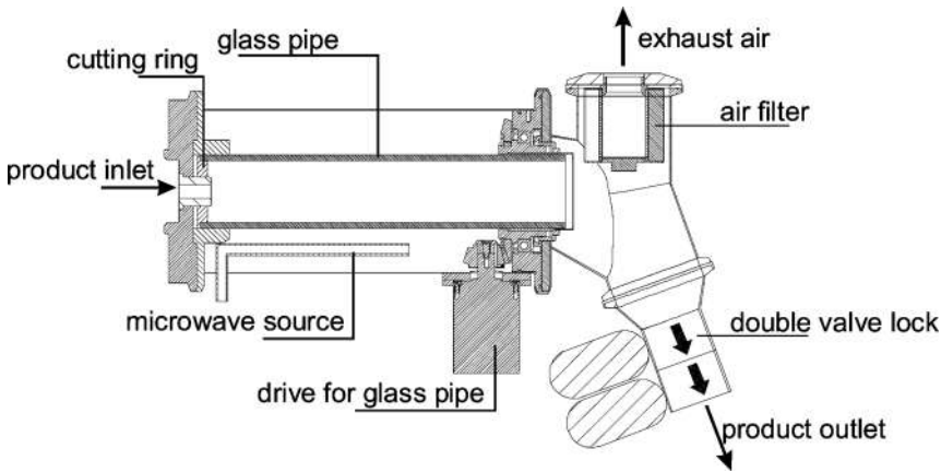
Figure 13 Sectional sketch of a microwave dryer.
