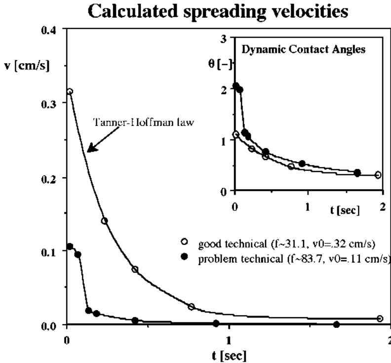
Figure 18 Dynamic imaging of drop wetting, and its impact on continuous pan granulation: (A) Dynamic image of a drop wetting into a formulation, with good active ingredient. (B) Comparison of surface spreading velocity and dynamic contact angle vs. time for good and bad active ingredients or technical. Bad technical required reduced production rates. (From Ref. 4.)
