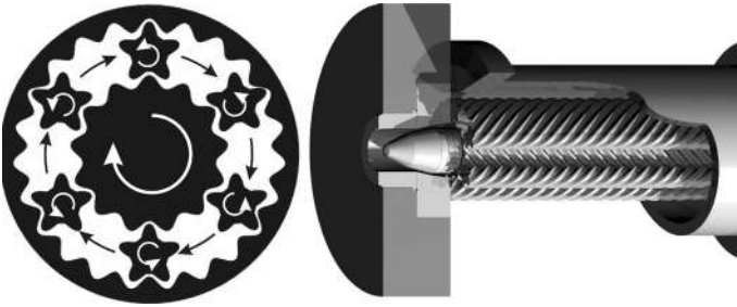
Figure 10 Appearance of a planetary roller extruder. The arrows on the left side indicate the movements during extrusion.
