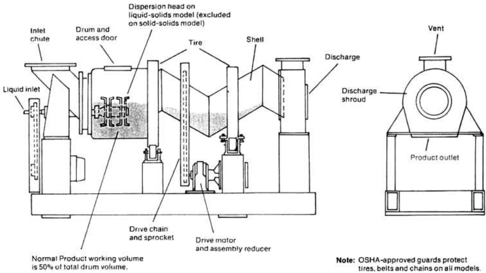
Figure 11 Schematic of a Zig-Zag, which is an example of a continuous granulating machine. (Courtesy of Patterson-Kelley Co., Division of Harsco Corp., East Stroudsburg, PA.)
