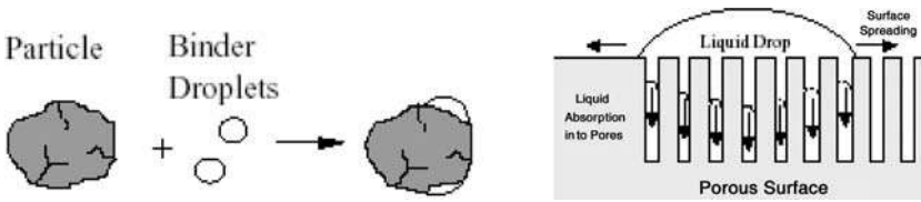
Figure 13 Stages of wetting for coarse powder compared to drop size. (From Ref. 5.)
